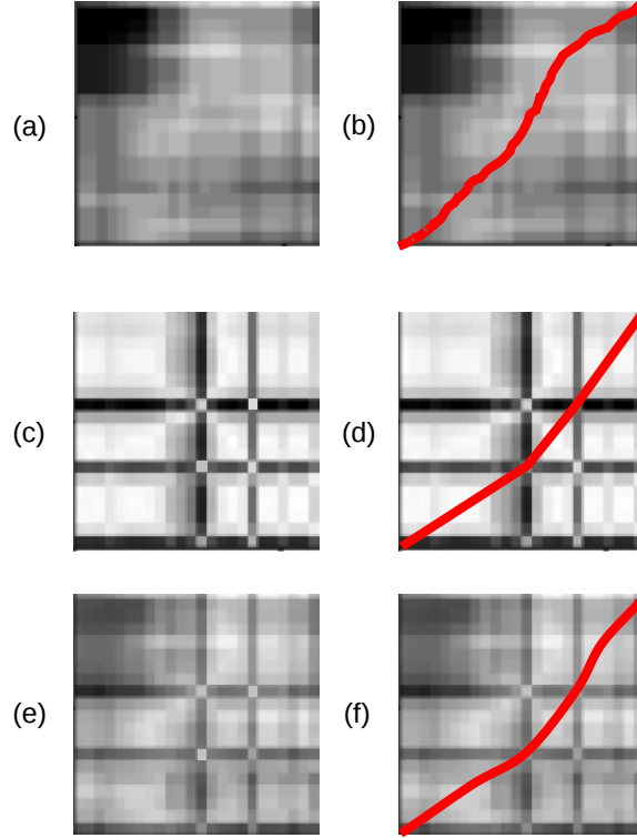
Figure 3.3: Excerpts from cost matrices and corresponding warping paths computed with DTW (a)/(b): C_{\text{CHROMA}} , (c)/(d): C_{\text{ACT}} , (e)/(f): \alpha C_{\text{CHROMA}} + (1 - \alpha) C_{\text{ACT}} , with \alpha = 0.5 .
