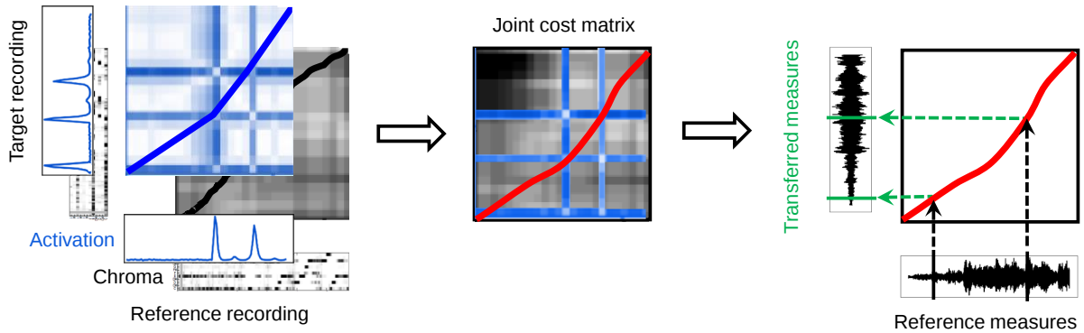
Figure 3.1: Overview of the combined approach integrating activation functions into a conventional chroma-based synchronization pipeline. The cost matrix computed with activation cues (blue) yields a grid-like structure to guide the alignment of musical events, whereas the chroma-based cost matrix (black) accounts for the robustness of the overall synchronization. The resulting warping path (red) is used for transferring measure positions.
