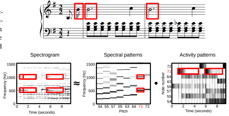
Figure 8.2: Decomposing the magnitude spectrogram of an audio excerpt of Chopin’s Prelude Op. 28 No. 4 into template and activation matrices. The information related to the note number p = 71 (B4) is indicated by the red rectangular frames.
